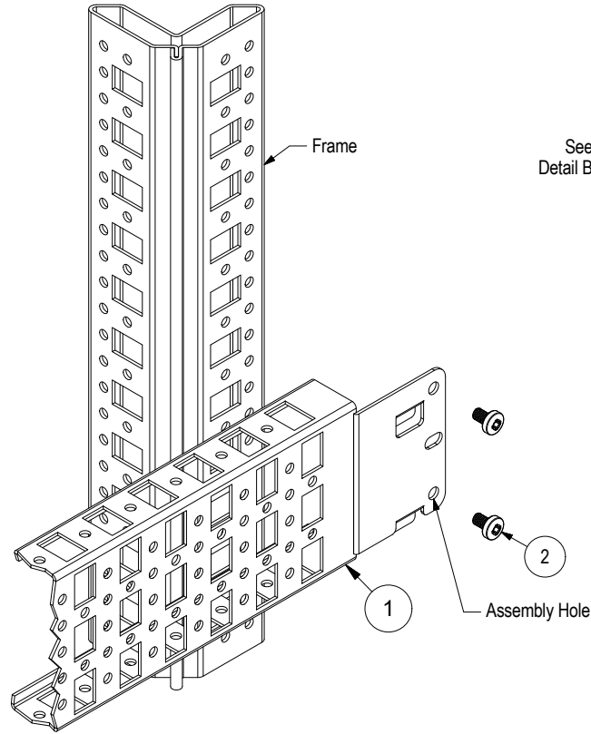
DETAIL B
