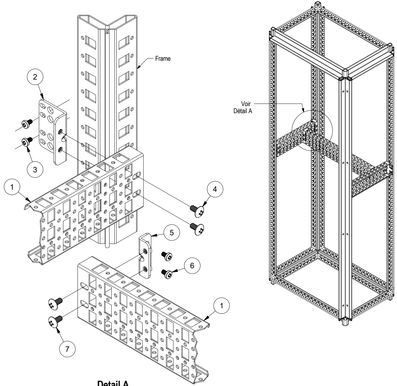
Detail A
