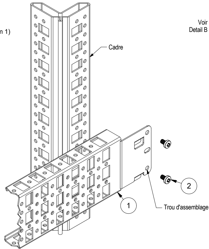
DETAIL B
