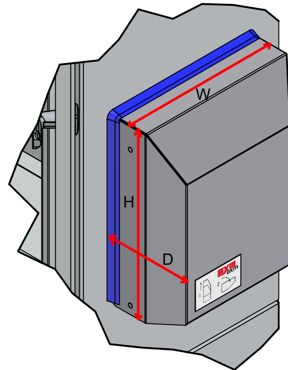
DETAIL A
